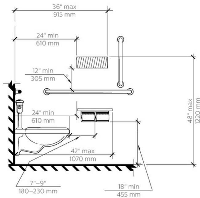
Figure 8 ADA Design guide for a toilet
